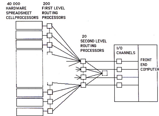
FIG. 2. GENERAL LAYOUT.
