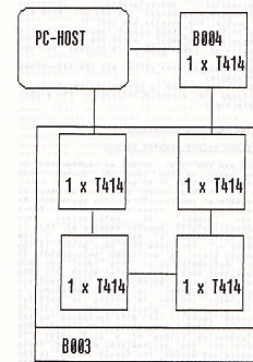
Fig. 2. Hardware Configuration.
