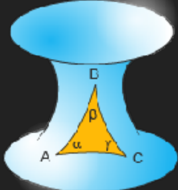
Hyperbolic Surface
